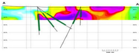
Vertical section cut from the 3D model
