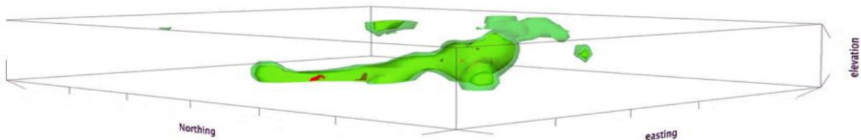
3D resistivity iso-surface produced using inversion modelling results
